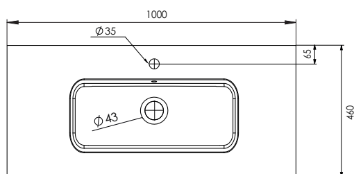
LUSO wastafel cast marble 100 cm
